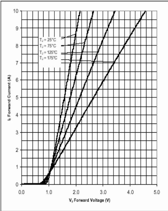
Figure 1. Forward Characteristics
