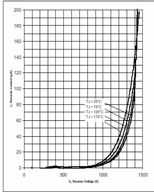
Figure 2. Reverse Characteristics
